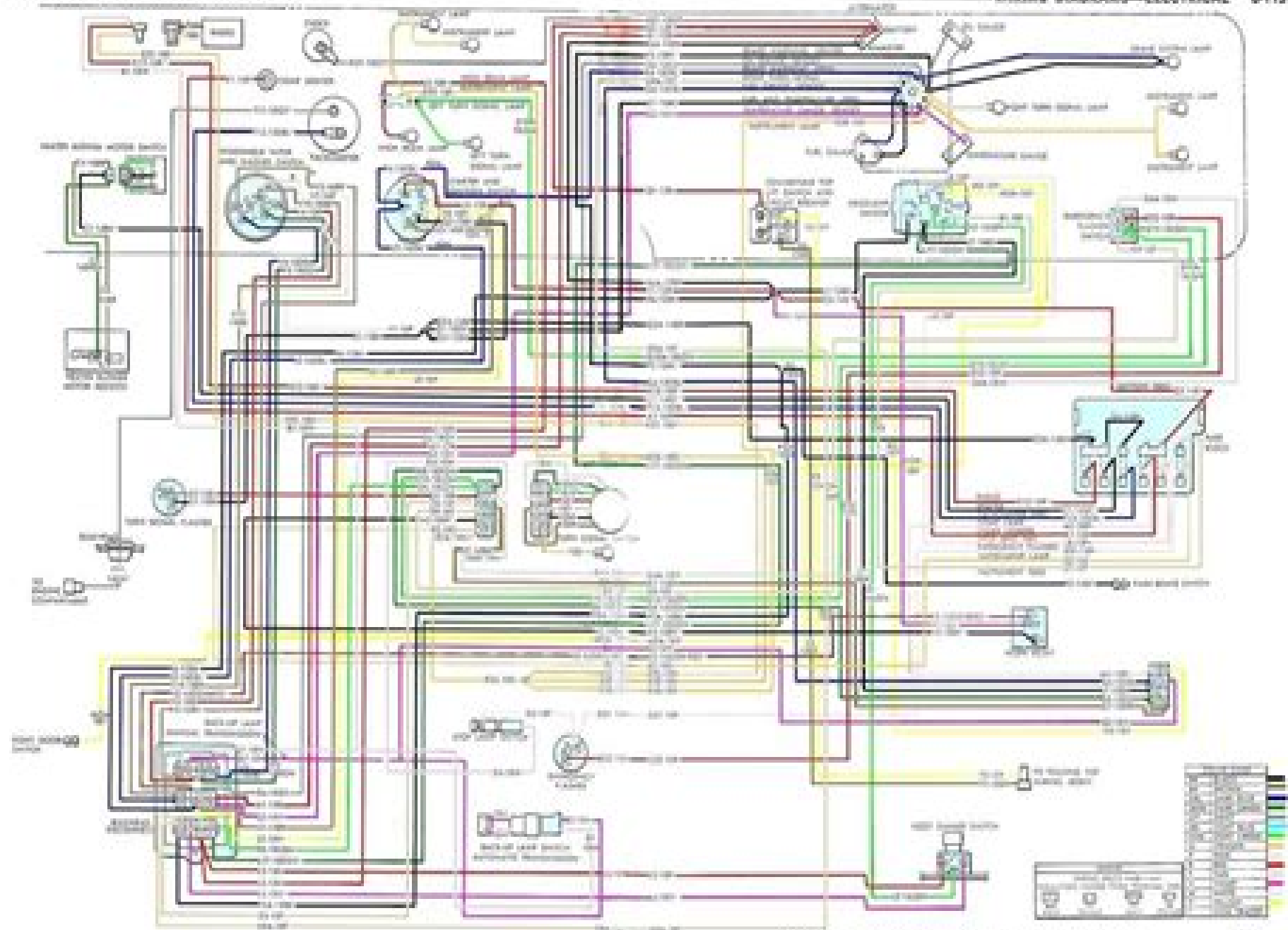
Fig. 7-Instrument Panel Wiring Diagram—Barracuda Model
