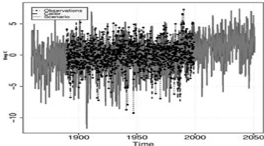
Fig. 1. Example of downscaled monthly 1890–1998 January mean temperature for Oslo-Blindern derived with clim.pact. The example is based on the ECHAM4/IPPC3 model and the IPCC IS92a-based GSDMO integration. (The GSDMO scenario includes the effects of greenhouse gases, tropospheric ozone, and direct plus indirect effects of industrial aerosols). The predictor used for calibration was gridded temperature described by Bengtsson [2001].
