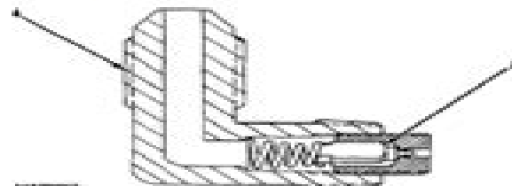
CONSTANT BLEED VALVE
