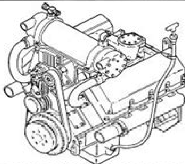
ENGINE, DIESEL, LIQUID COOLED V-TYPE, EIGHT CYLINDER, CUMMINS MODEL V903C W/CONTAINER (NSN 2815-01-399-6801)
