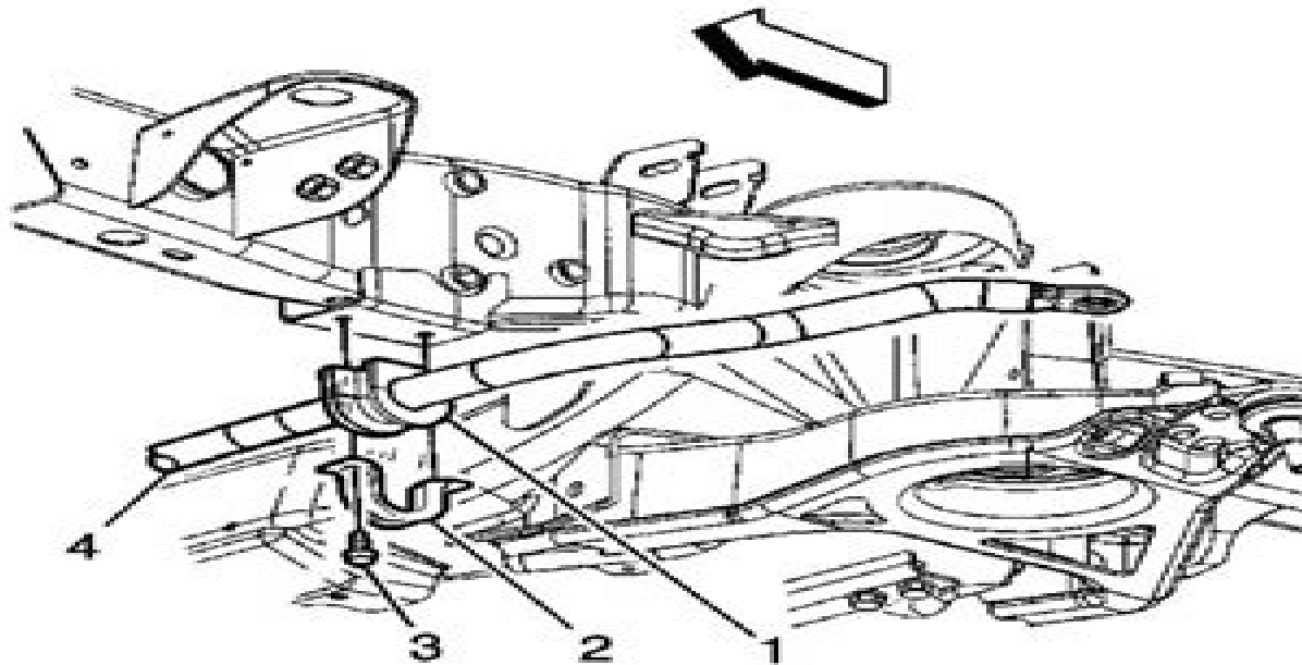
Fig. 3: Stabilizer Shaft, Bracket, Bolts & Insulators Courtesy of GENERAL MOTORS CORP.
