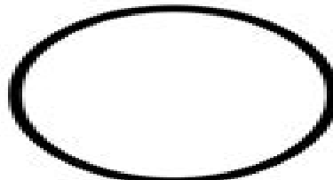
Neptune
