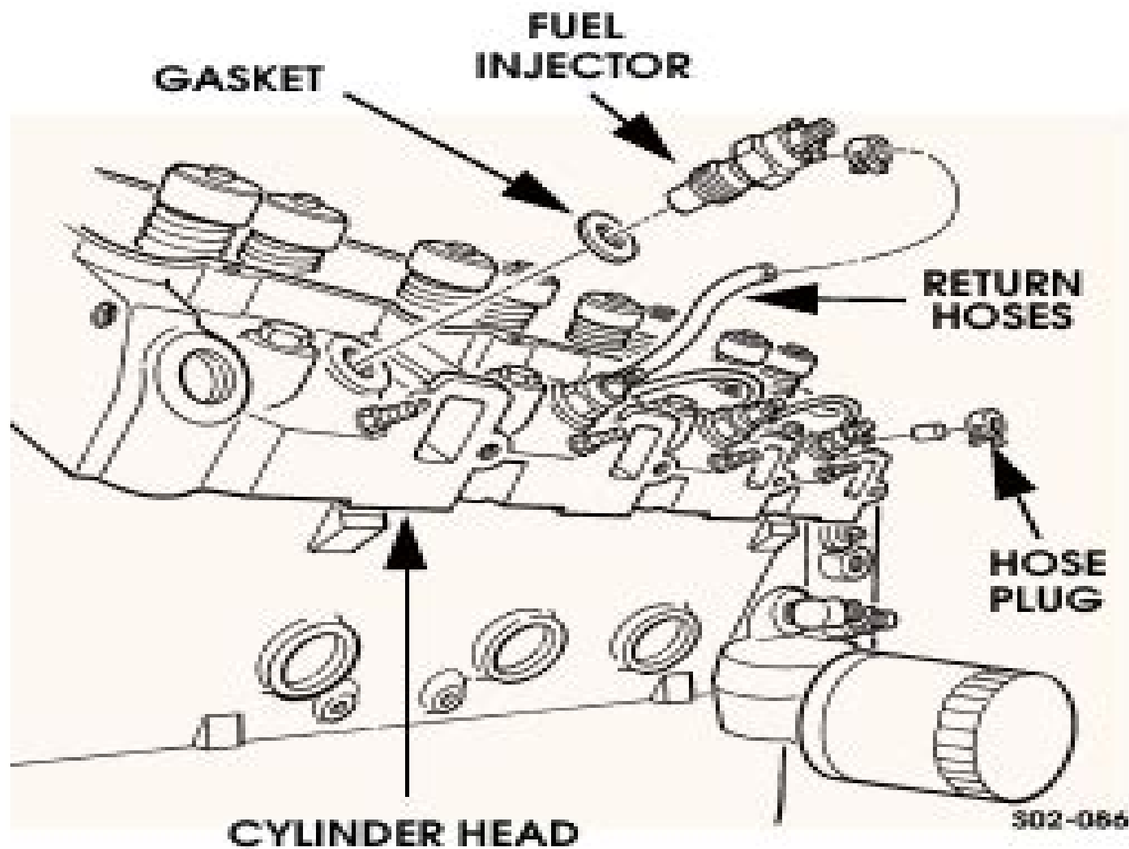
Figure 2-79: Fuel Injector Removal
