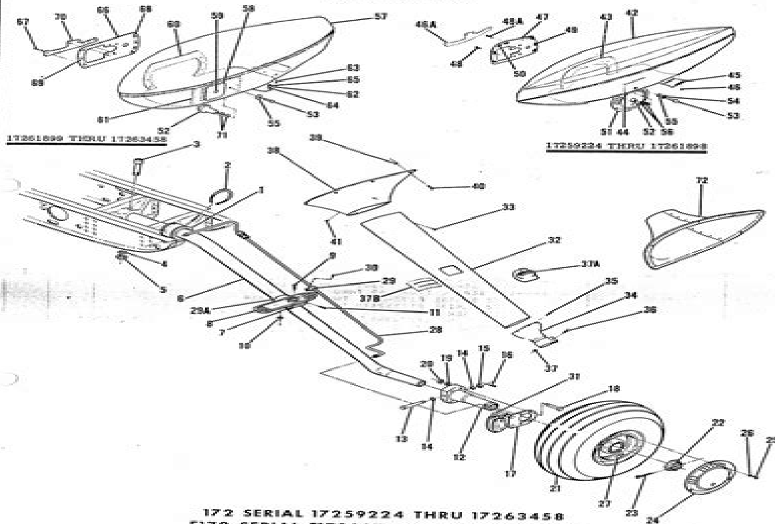
Figure 68. Main Landing Gear Installation.
