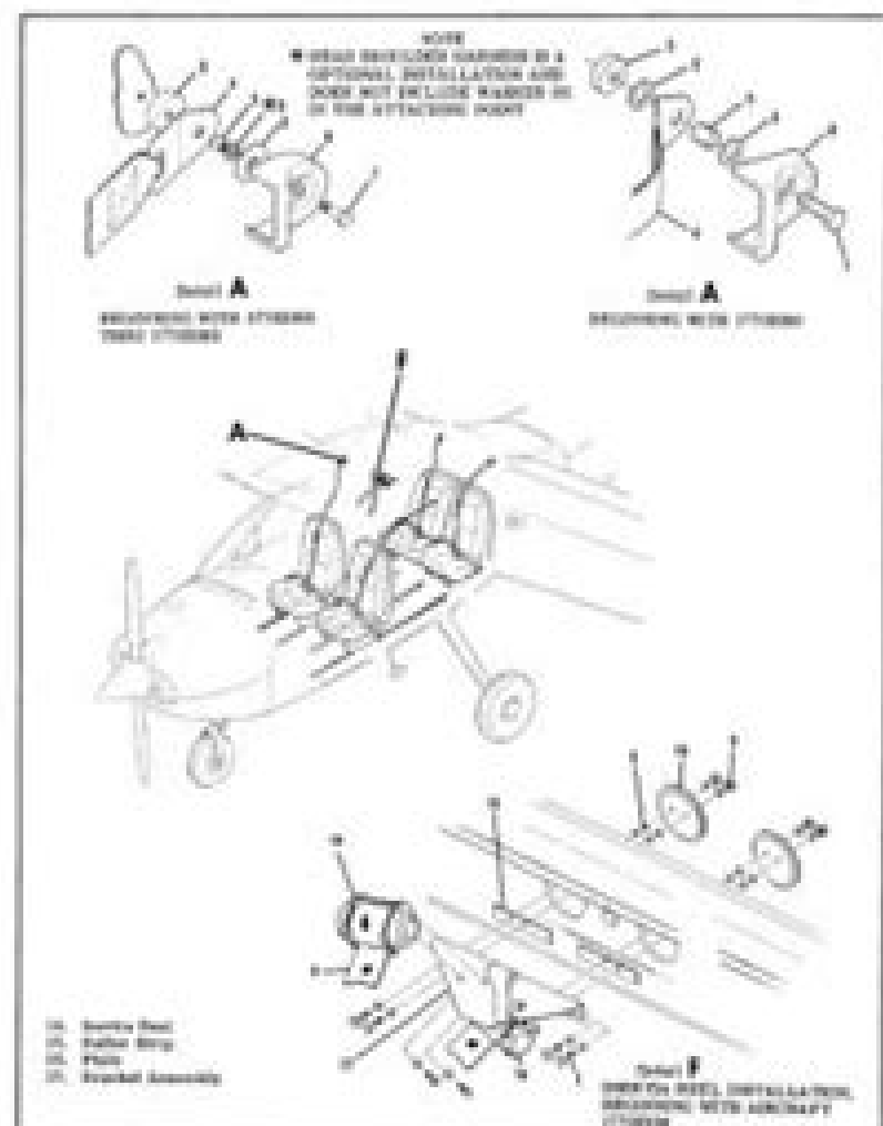
Figure 3-55. Seat belt and shoulder harness installation (Sheet 2 of 2)
