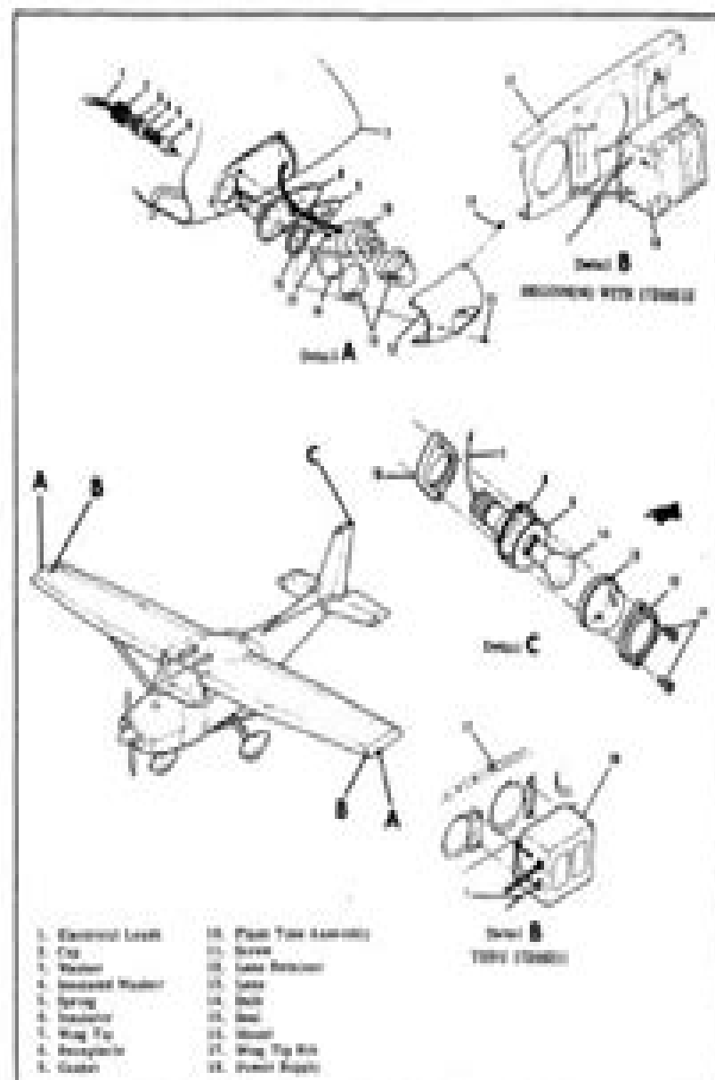
Figure 15-7. Navigation and Anti-Collision Strobe Light Installation
