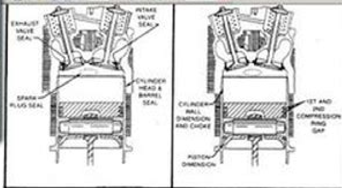
STATIC SEAL
