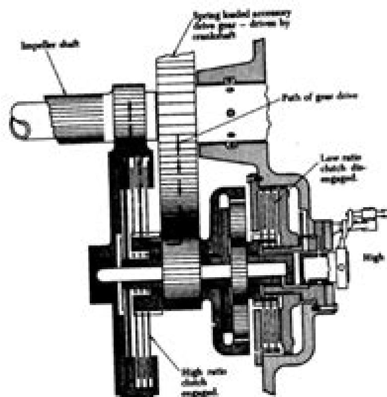
FIGURE 2-4. Schematic diagram of two-speed supercharger in high ratio.
