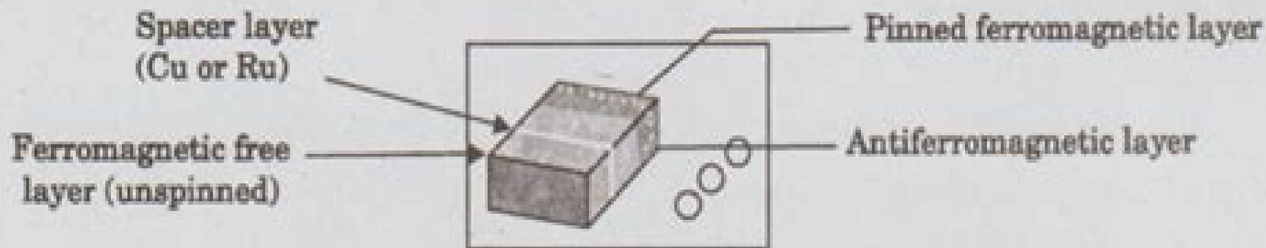
Fig. 2.35 (b) Spin valve
