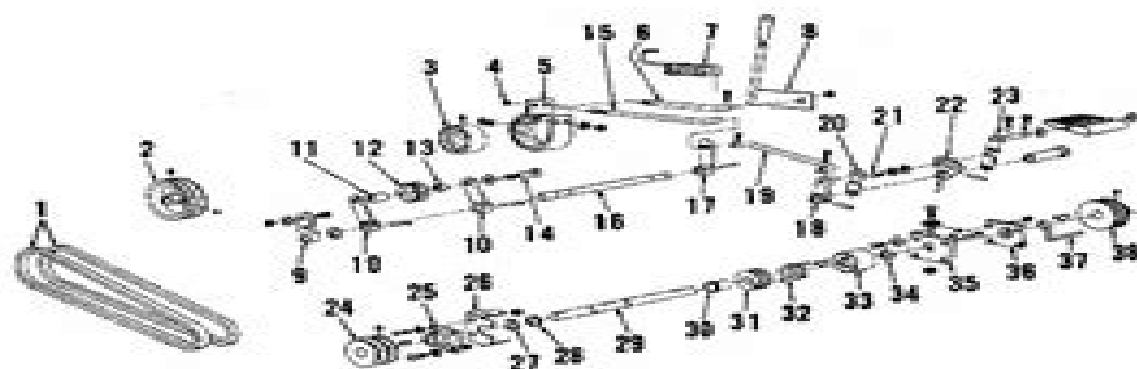
Fig. G11 — Exploded view of clutch-brake system used on Models 754, 755, 780, 53000, 53001 and 53008.
