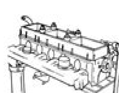
FIG 1-34 Compression frame installation
