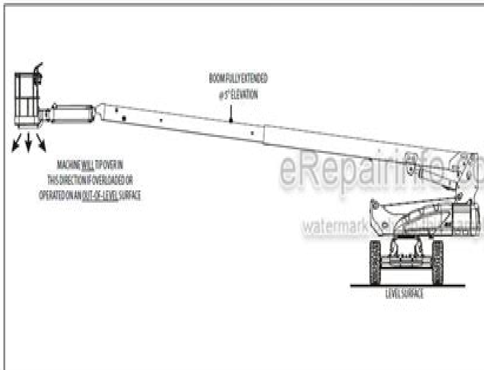
Figure 4-1. Position of Least Forward Stability
