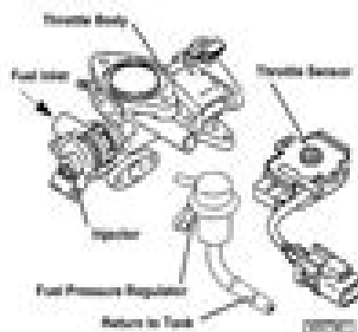
FD300V Throttle Body
