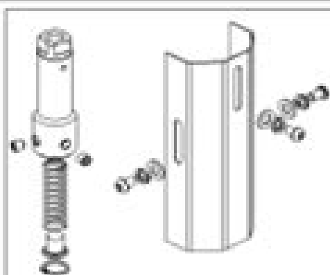
Exploded diagram of the RB32 safety guard schematic and included RB334 3/4" arbor.
