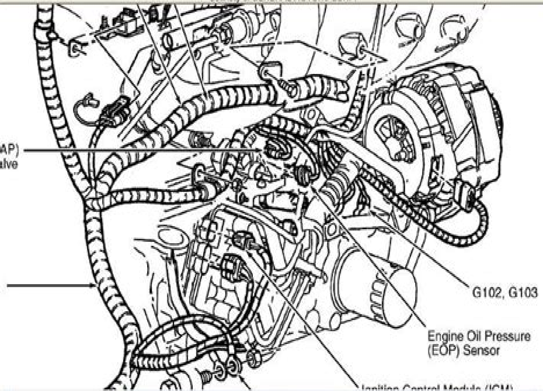
Fig. 3: Right Side Of Engine (2.2L VIN 5) Courtesy of GENERAL MOTORS CORP.
