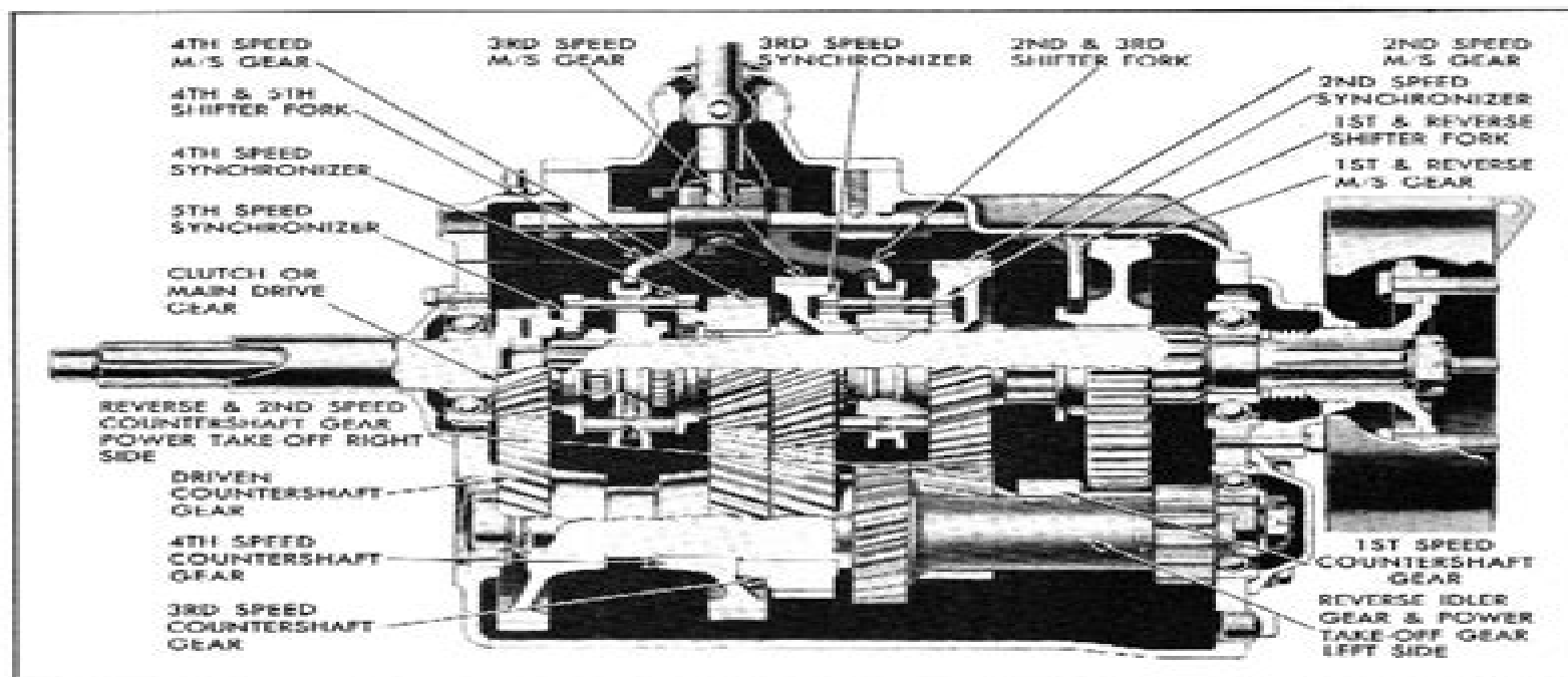
Fig. 3—Cross section (Spicer)
