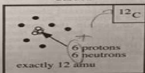
Carbon
