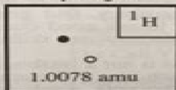
Hydrogen
