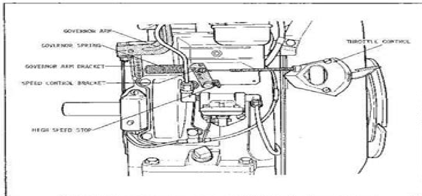
FIGURE 8. VARIABLE SPEED GOVERNOR
