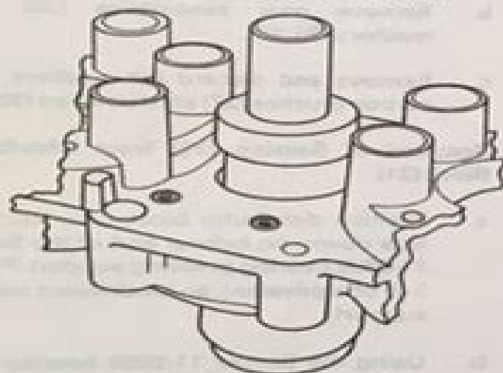
Figure 2-4 Bearing Pressing Tools in Proper Position
