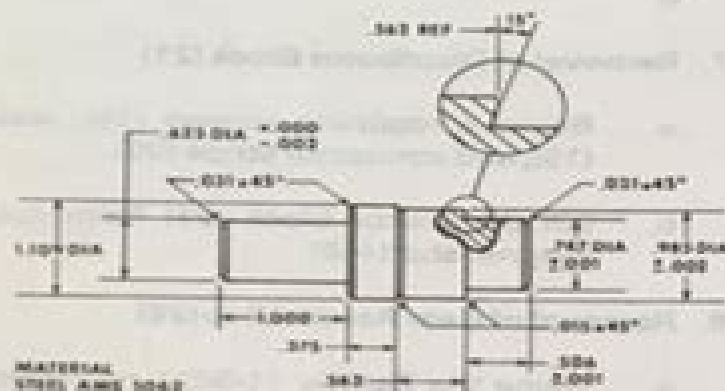
Figure 2-3 11-9998 Bearing Pressing Tool
