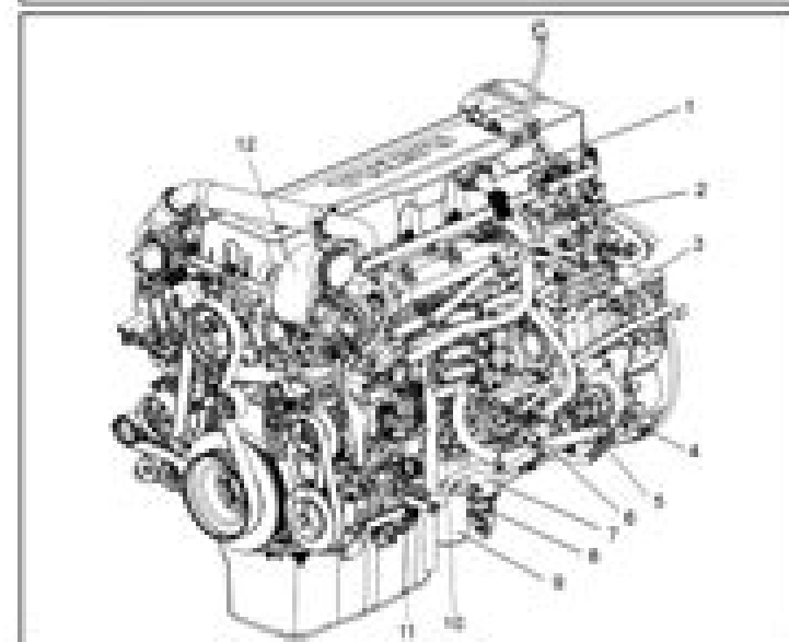
Figure 1. Front view, 4x2, 6x4 and 8x4 (D13) (1/1)
