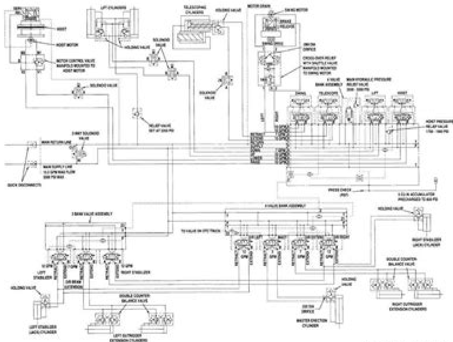
FO-8: Hydraulic Schematics (MMAET Crane) (Sheet 8 of 10)
