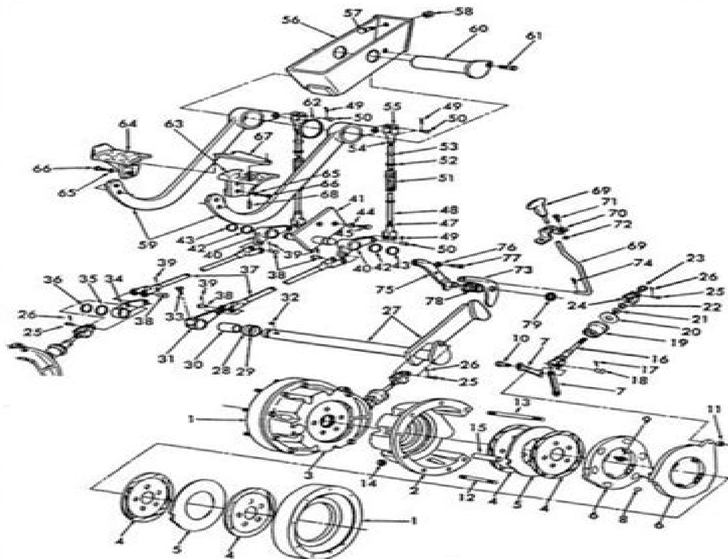
FIG. 2A1 - BRAKES &amp; BRAKE CONTROLS
