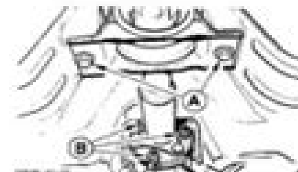
Fig. 45. Fixature of driveshaft. A - Centre bearing balls B - Transmission output flange nuts
