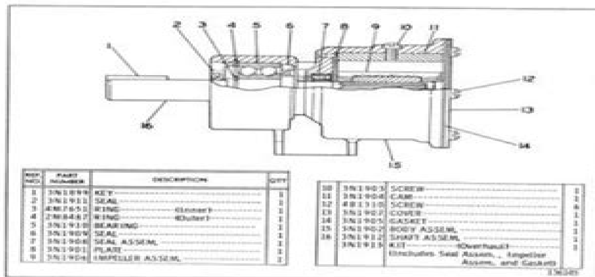
2N3084 SEA WATER PUMP ASSEMBLY Part of Sea Water Auxiliary Pump and Lines
