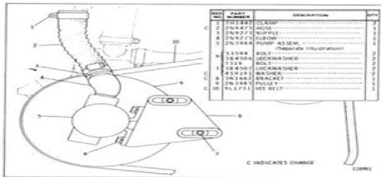
SEA WATER AUXILIARY PUMP AND LINES (2N5533 N/S)
