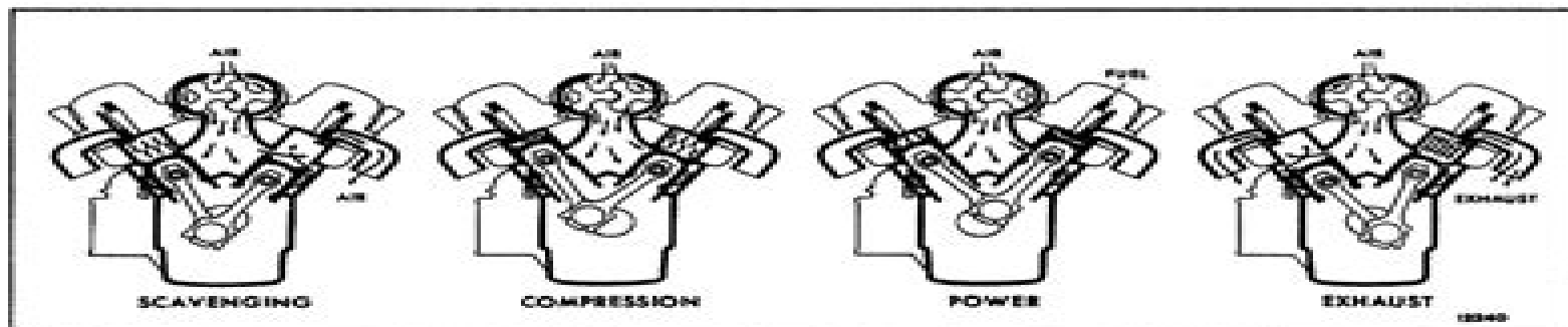
FIG. 1 - The Two-Stroke Cycle
