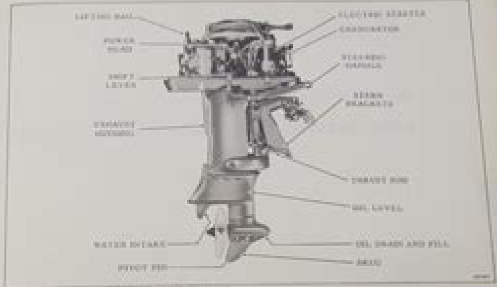
Figure 1-1. Starboard Side, 21 HP Extrude Motor
