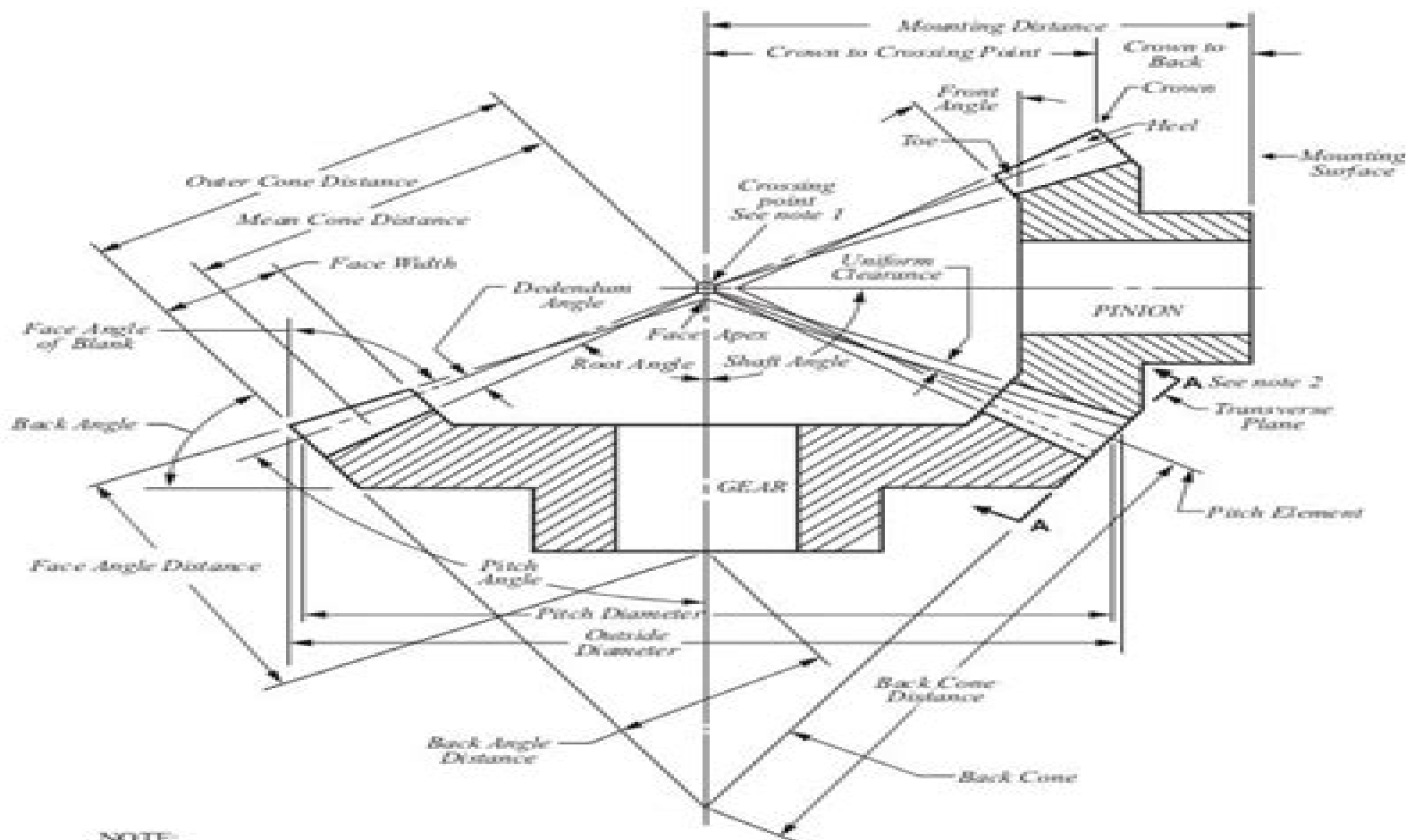
Figure 9. Bevel Gear Nomenclature – Axial Plane
