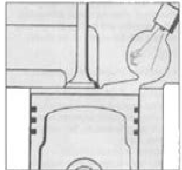
Injection into turbulence chamber
