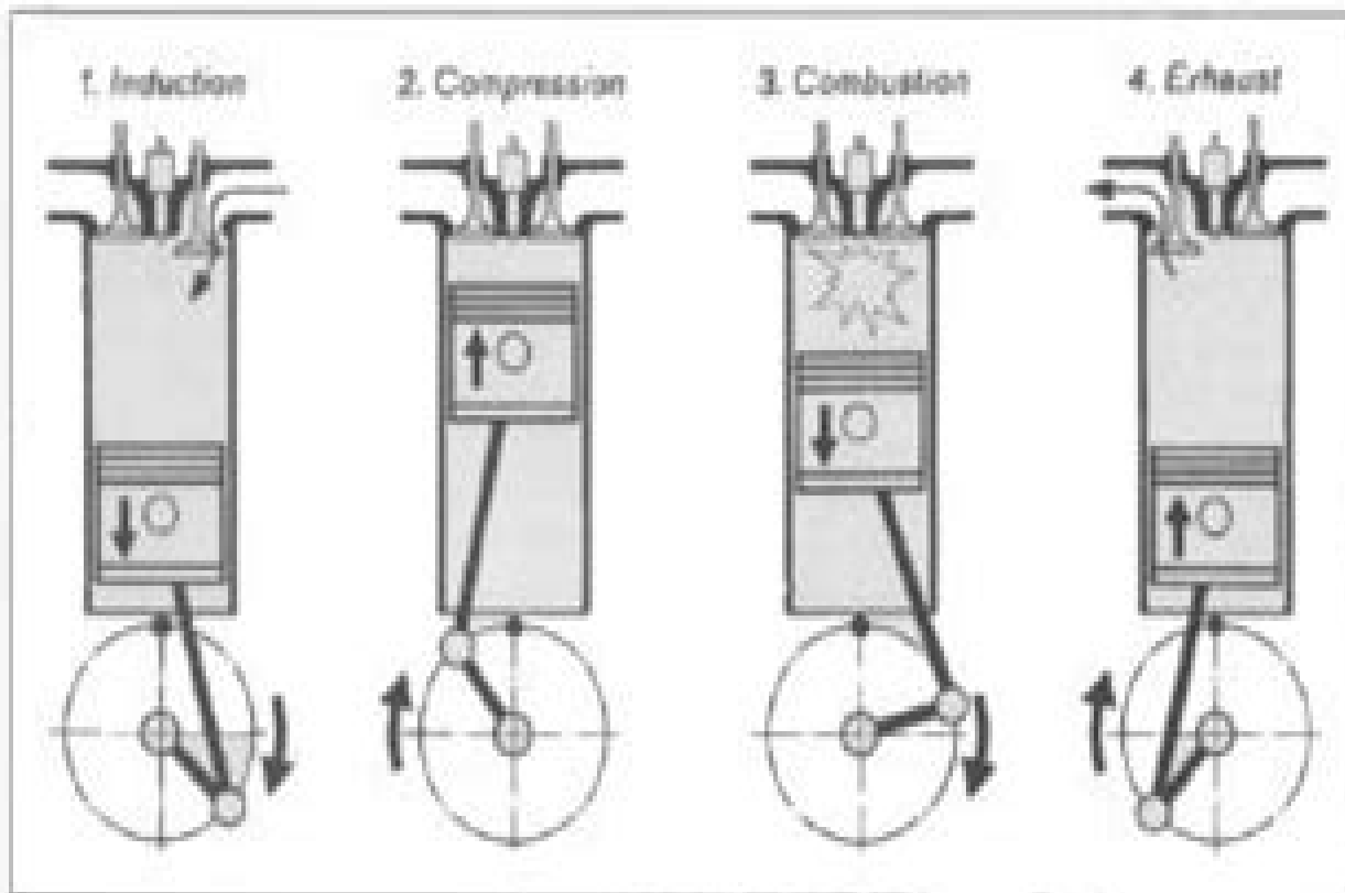
Four-stroke diesel cycle
