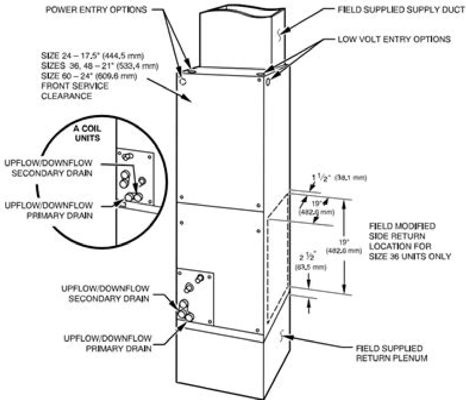
Fig. 2 – Slope Coil Unit in Upflow Application
