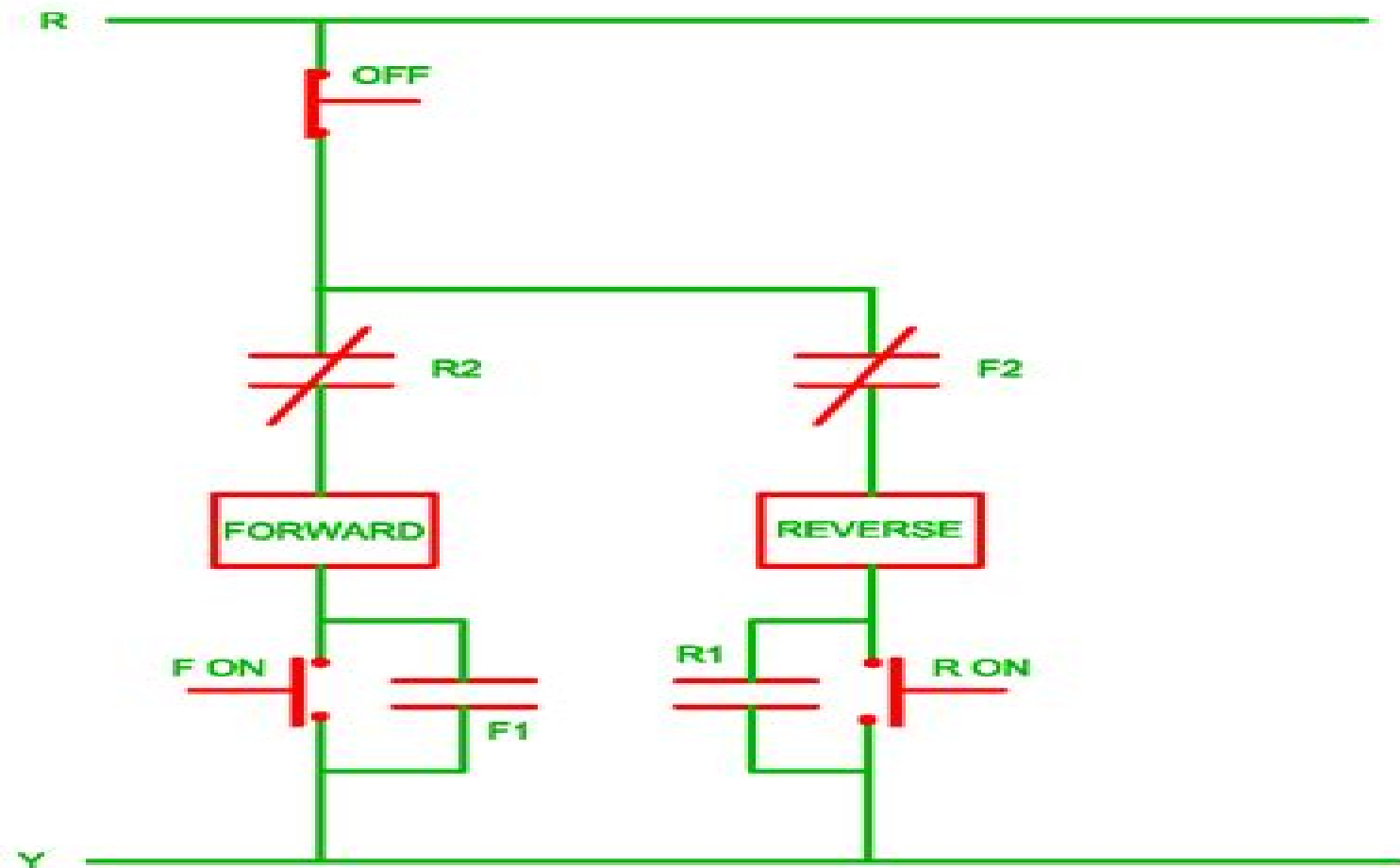
CONTROL CIRCUIT OF FORWARD REVERSE STARTER
