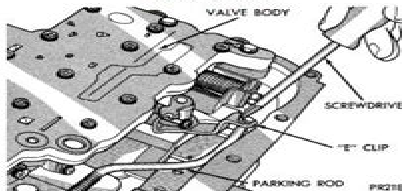
Fig. 50 Remove Parking Rod E-Clip
