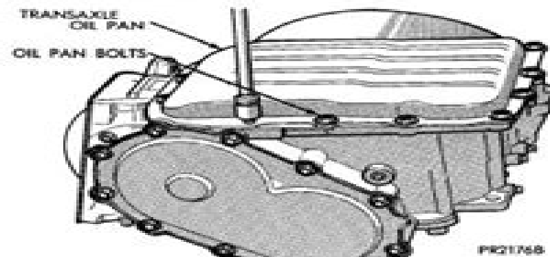
Fig. 46 Transaxle Oil Pan Bolts
