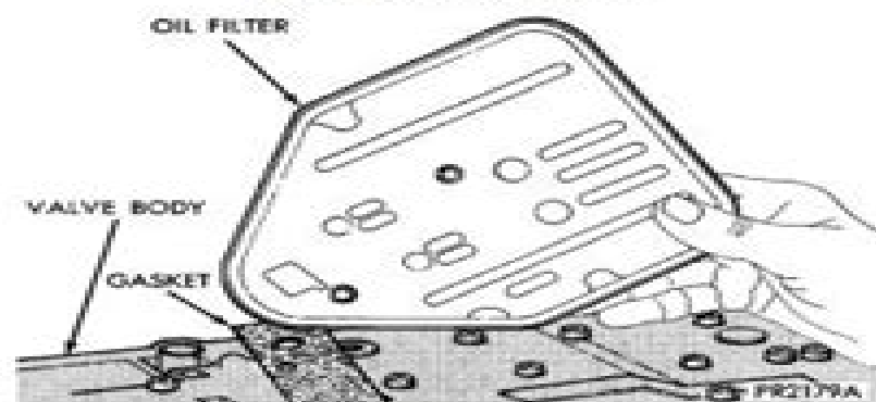
Fig. 49 Oil Filter
