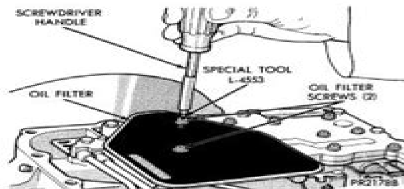
Fig. 48 Oil Filter Screws
