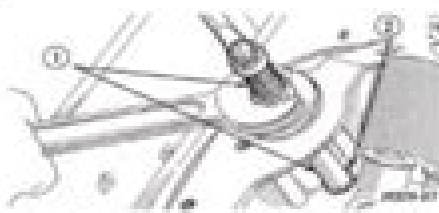
Fig. 43 Removing Distributor Driveshaft Bushing 1 - SPECIAL TOOL C-502 2 - BUSHING
