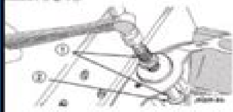
Fig. 44 Distributor Driveshaft Bushing Installation 1 - SPECIAL TOOL C-500 2 - BUSHING
