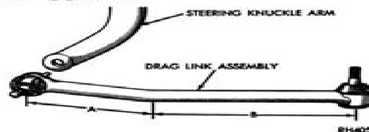
Fig. 18 Correct Drag Link Installation
