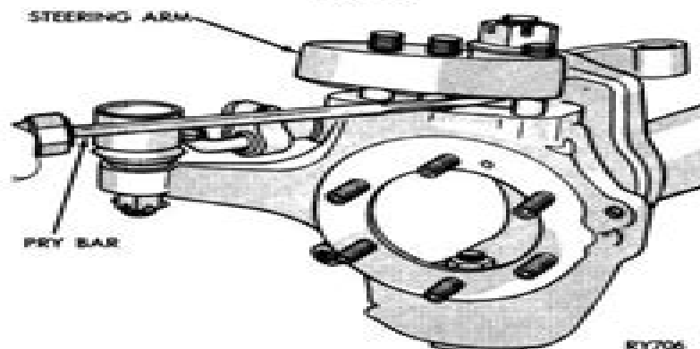
Fig. 17 Steering Knuckle Arm Removal
