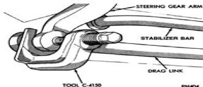
Fig. 16 Drag-Link Ball Stud Removal With Tool C-4150
