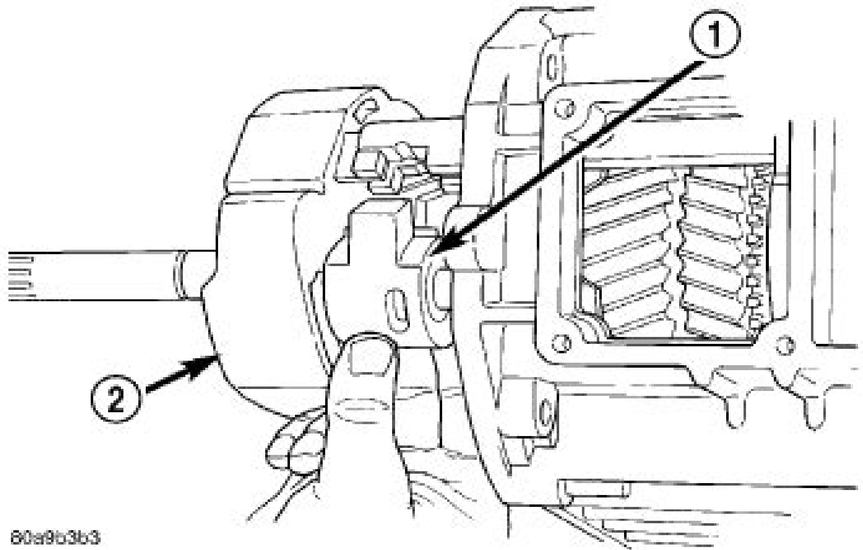
Fig. 15 SHIFT SHAFT LEVER AND BUSHING
