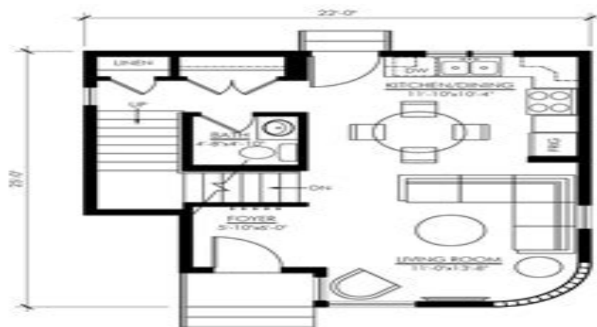
MAIN FLOOR PLAN - 489 SQ. FT. NORMANDIE - 945
