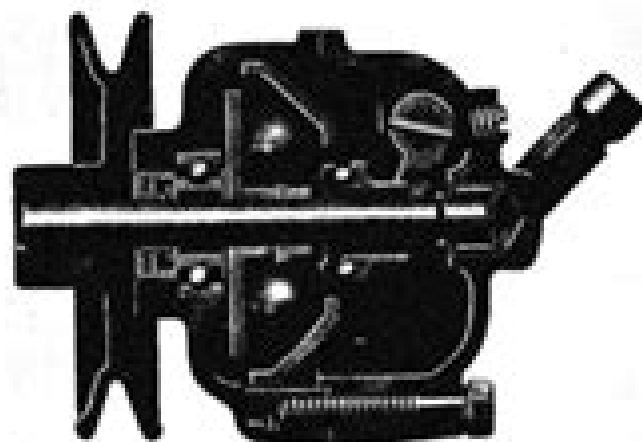
FIG. 13—GOVERNOR
