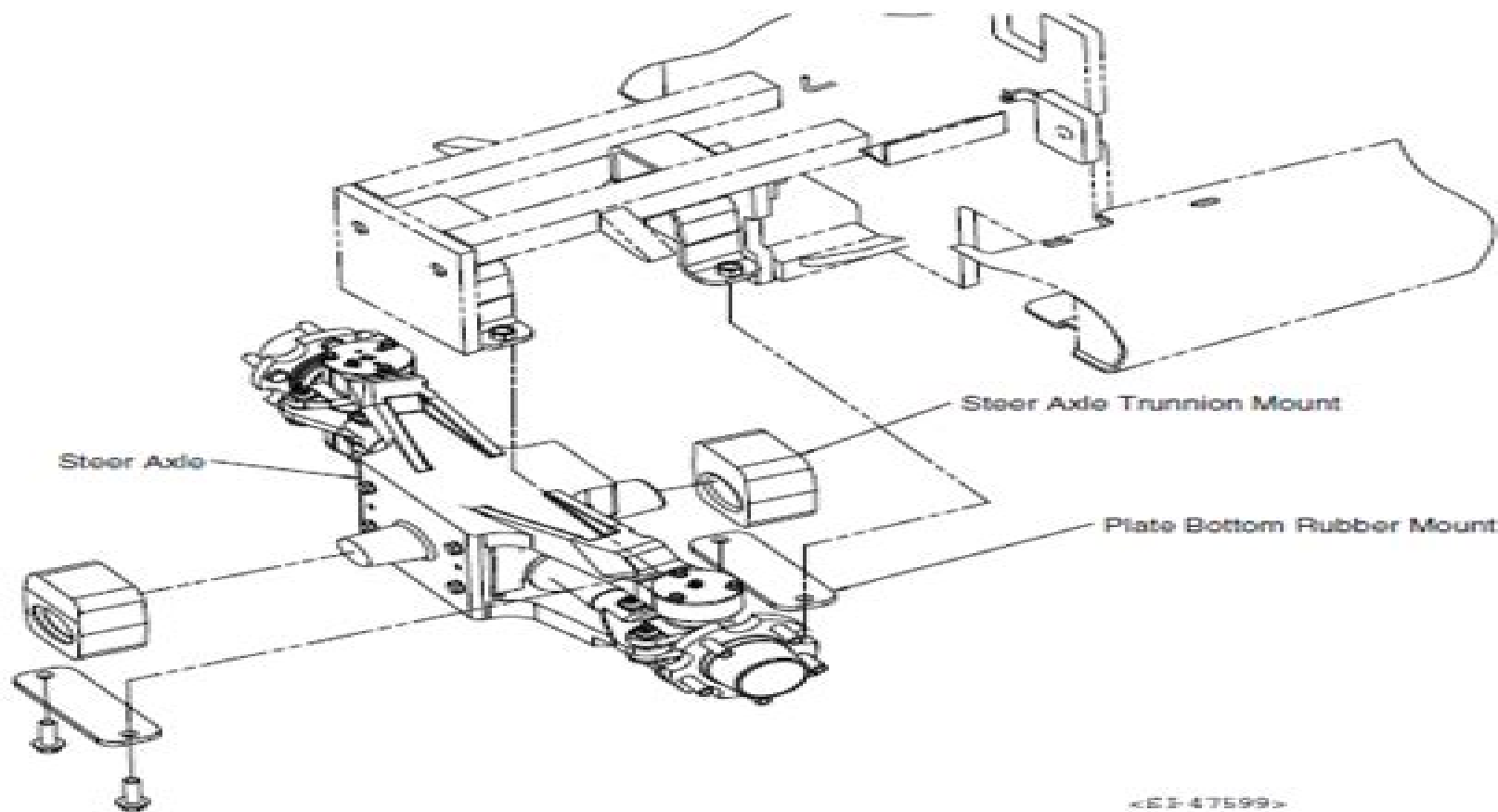
Steer Axle and Mounting
