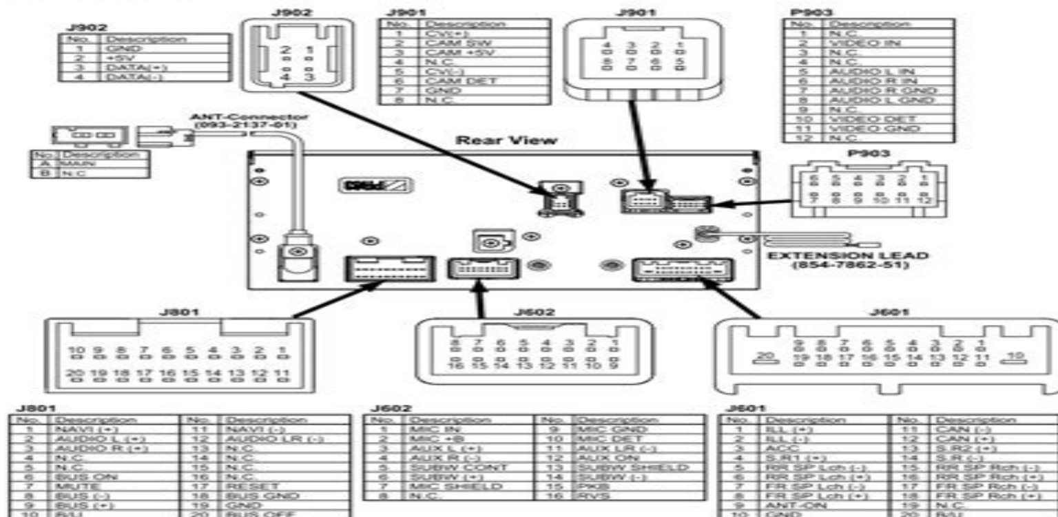
20 pin Nissan Head Unit Audio main connector
