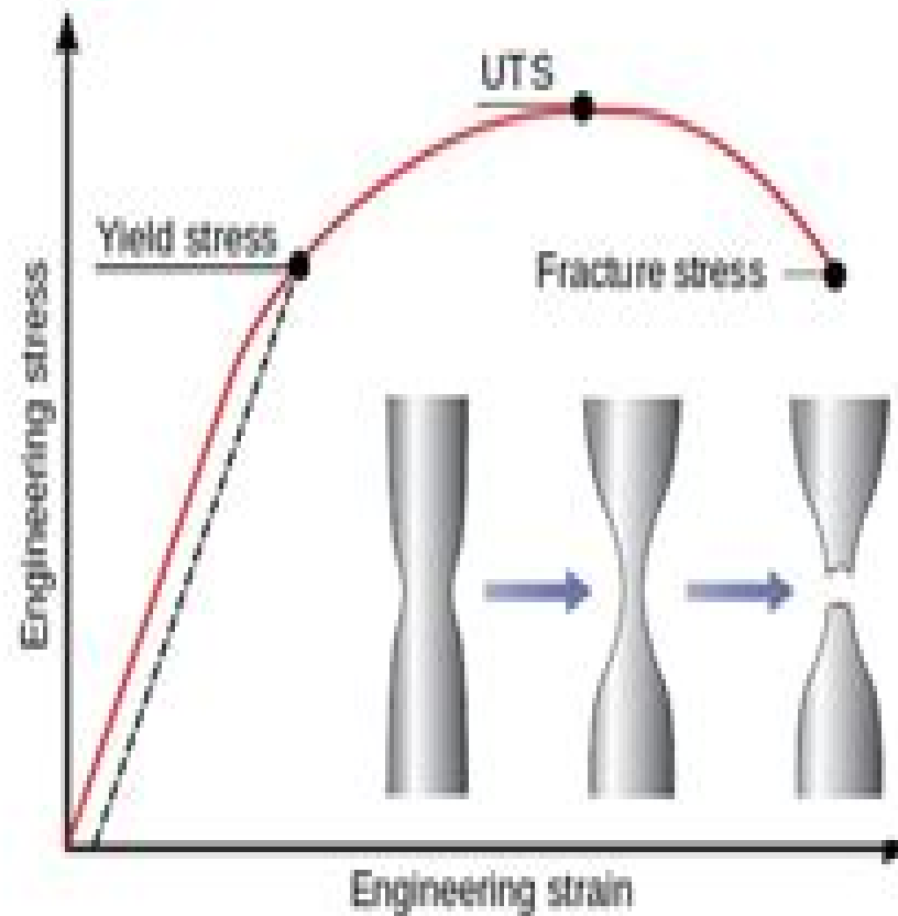
Stress - Strain Diagram
