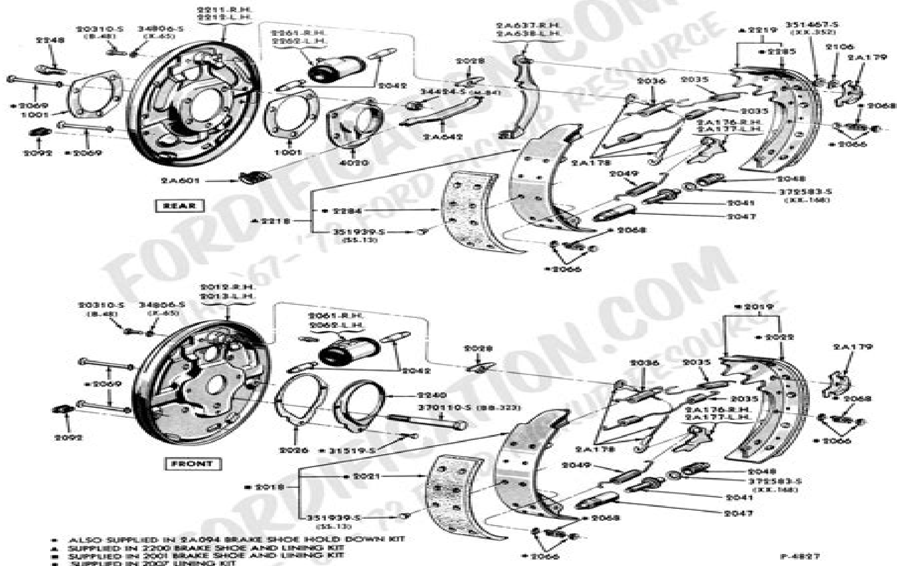
FRONT & REAR BRAKES - SELF ADJUSTING - TYPICAL 1964/72 E100/200, F100 (4 x 2) P100 1967 F100 (4 x 4), F250, P350/400
