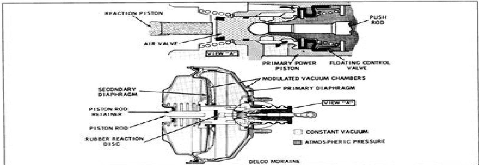
Fig. 5D-5 Releasing Position
