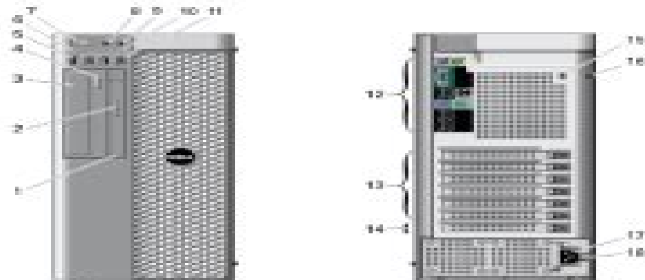
Figure 1. Front and Back View of T3610/T5610
