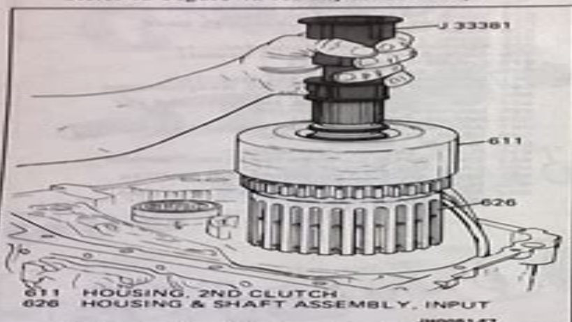
Figure 17 2nd Clutch and Input Clutch
