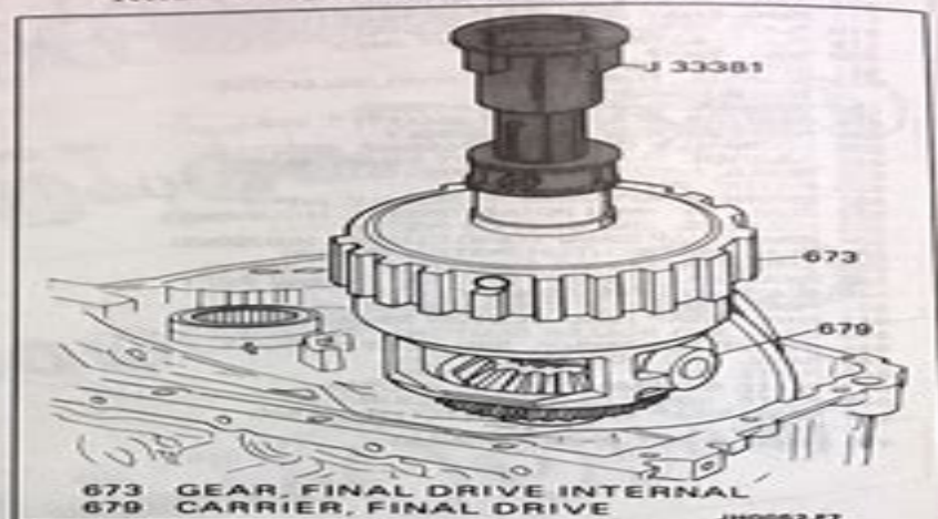
Figure 18 Final Drive
