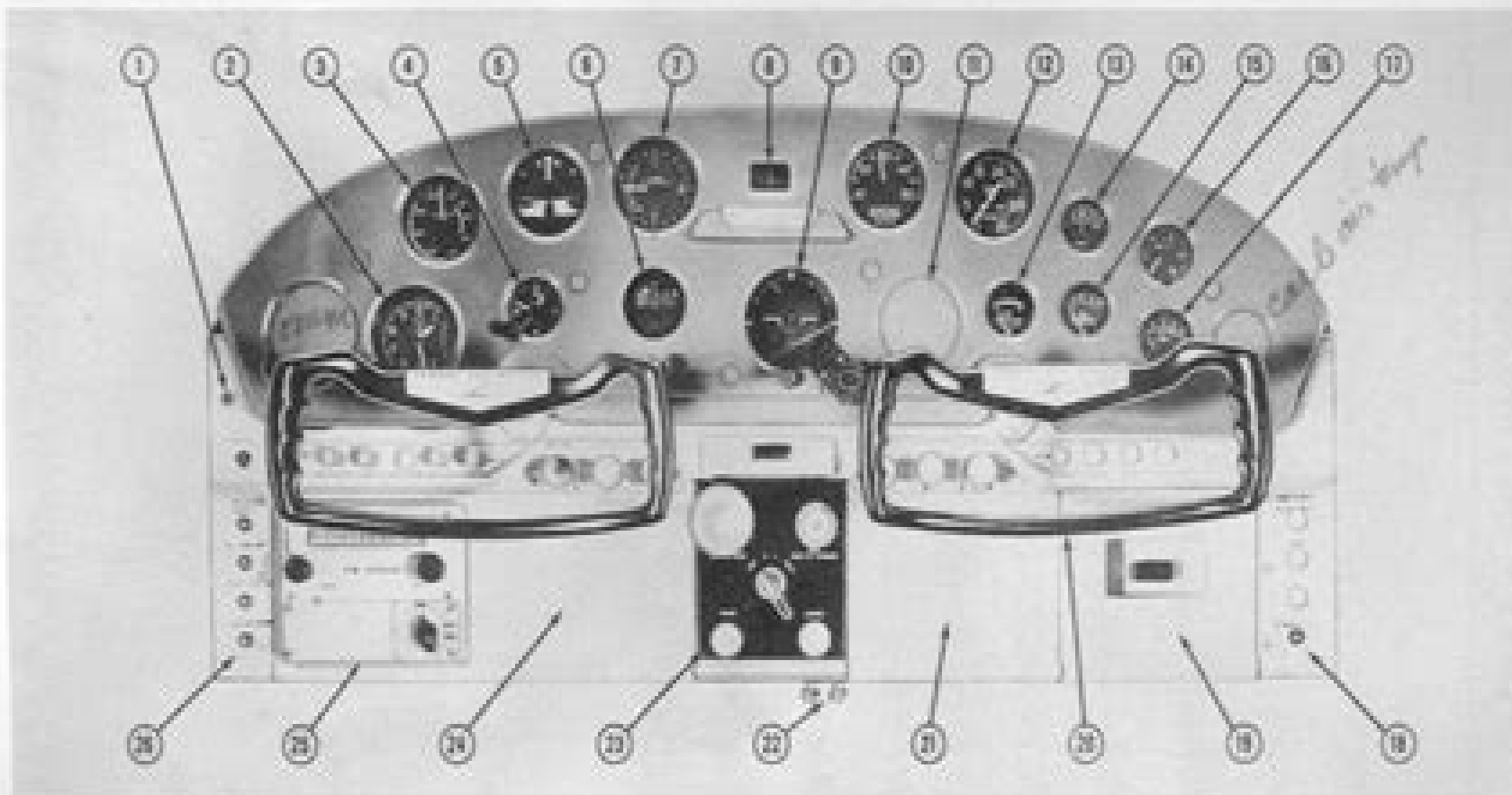
Figure 1. Instrument Panel
