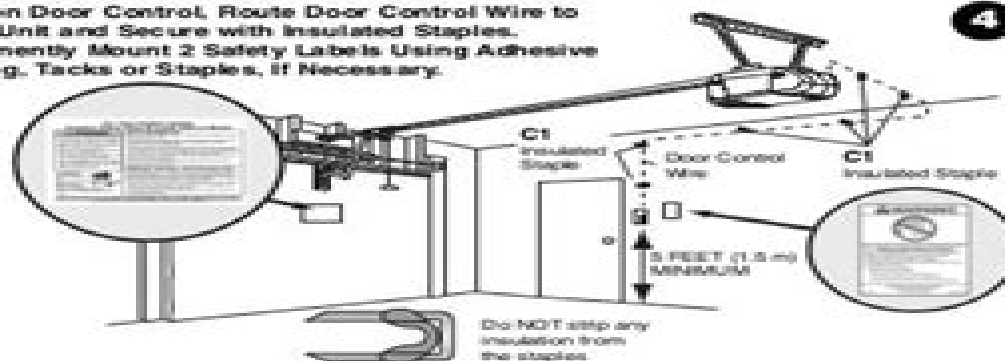
Multi-Function Door-Control
